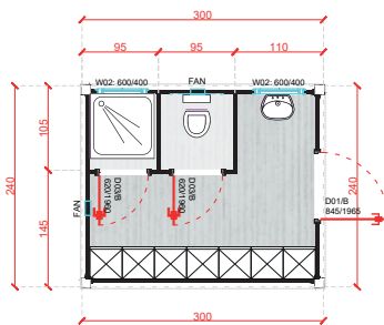
LC-A3000.2 300x240 cm
