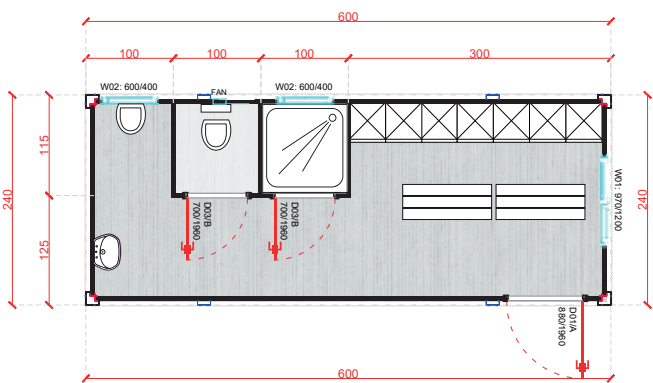
LC-11 20' 600x240 cm
