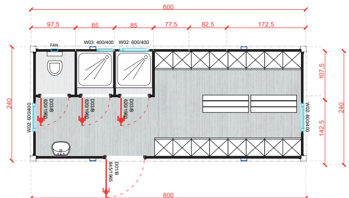
LC-A6000.2 20' 600x240 cm
