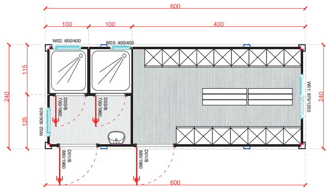
LC-13 20' 600x240 cm
