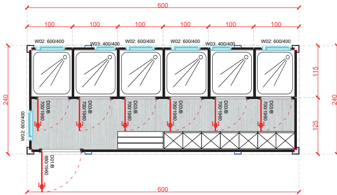
LC-12 20' 600x240 cm
