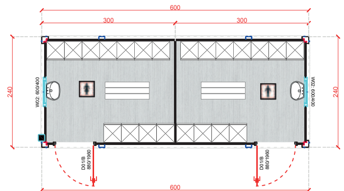
LC-16 20' 600x240 cm
