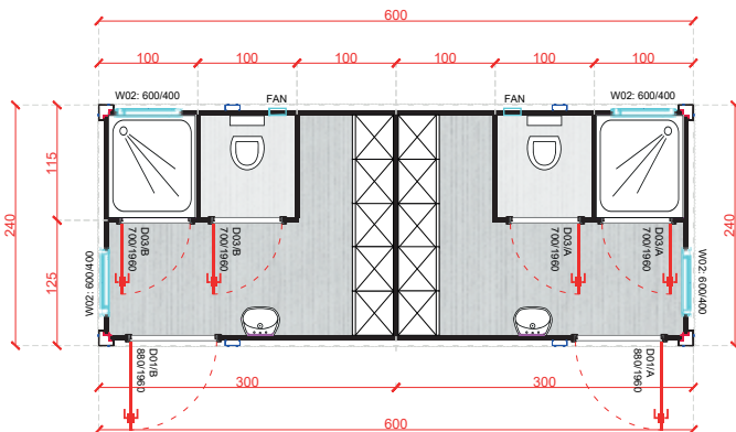
LC-15 20' 600x240 cm
