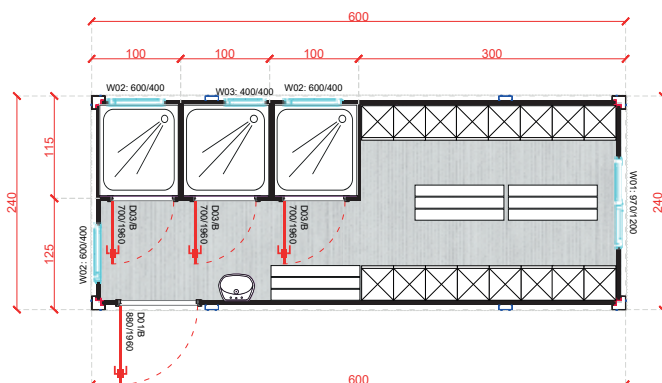
LC-10 20' 600x240 cm
