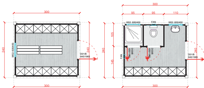
LC-A3000.1 300x240 cm
