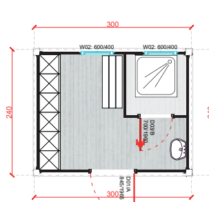
LC-A3000.3 300x240 cm
