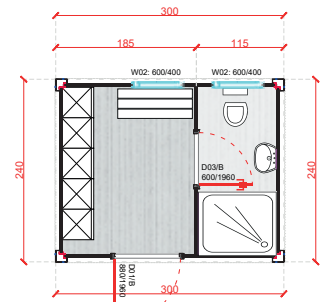
LC-A3000.4 300x240 cm
